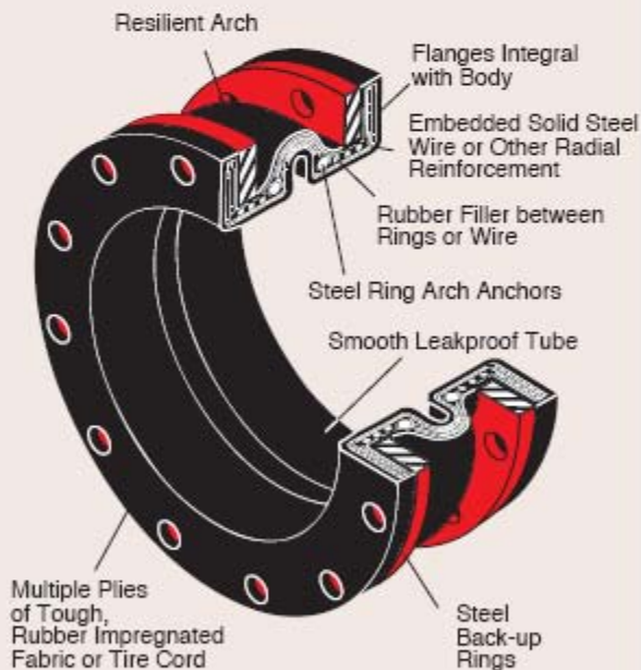
SERIES 500 SPOOL TYPE EXPANSION JOINT
